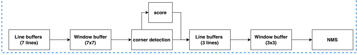
Figure 3.4: FAST corner detector submodule overview.
