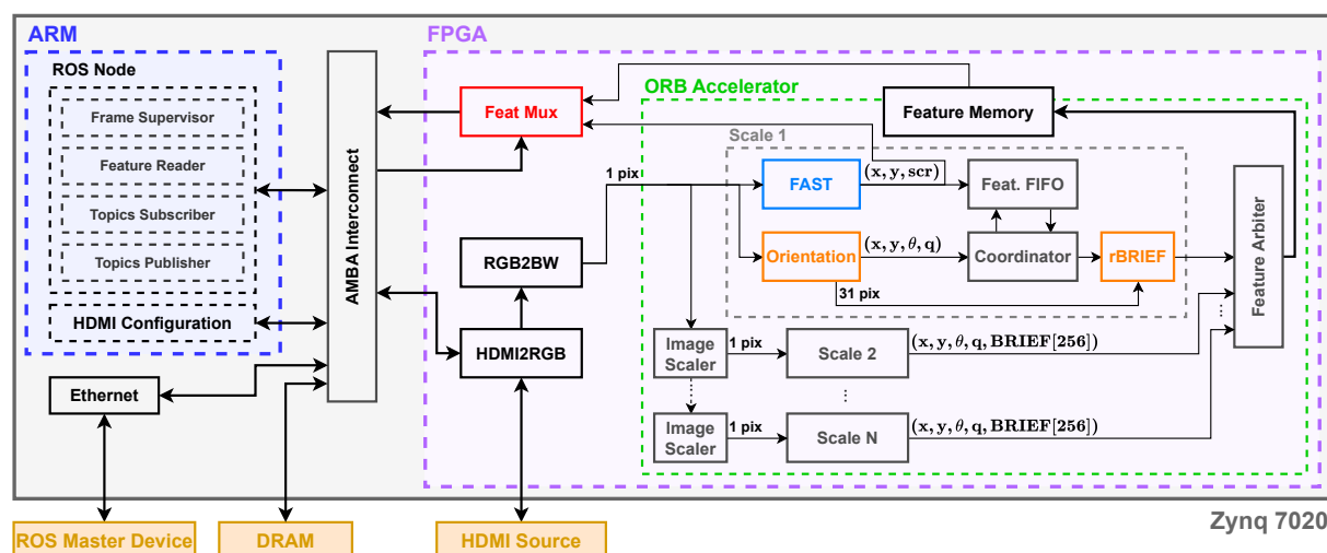
Figure 5.3: ORB accelerator device with added feature multiplexer (highlighted in red) for isolated FAST validation.
