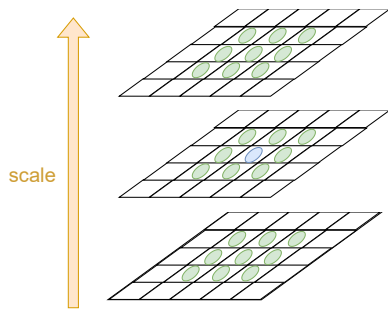
Figure 2.5: Extrema detection [1].
