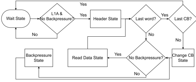
Fig. 4: Controller flowchart.
