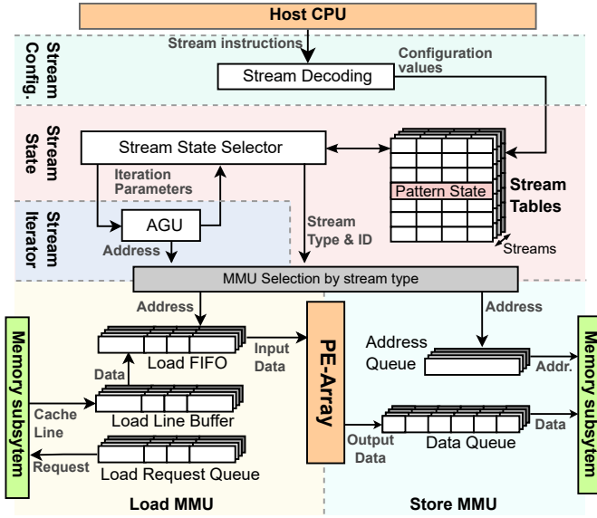
Fig. 2. Streaming engine architecture overview.
